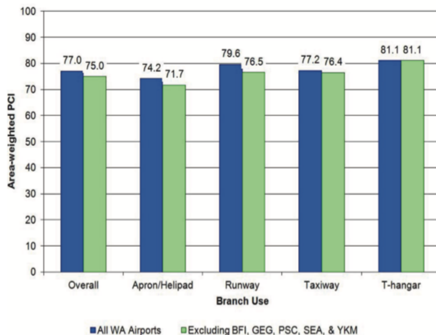
Figure 3: 2012 Area-Weighted Pavement Condition Index
